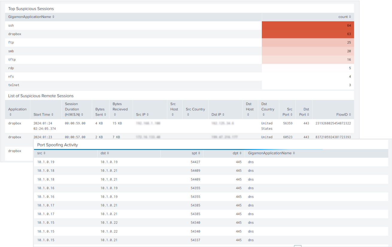
Figure 15. AMI metadata visualized in Splunk.
